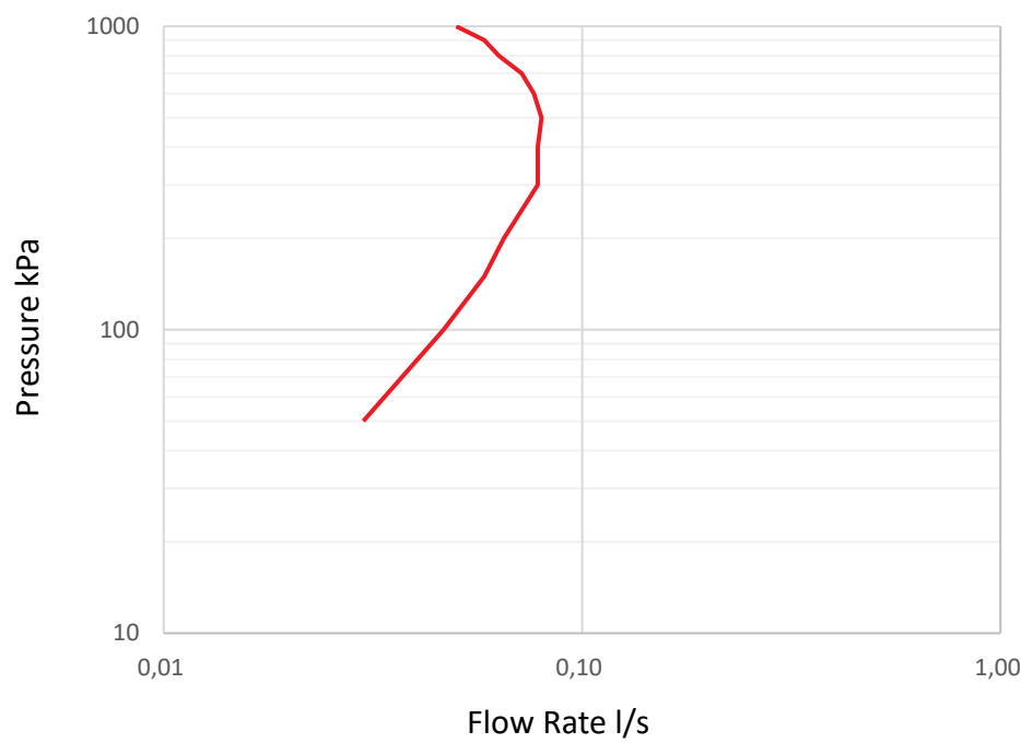
Flowchart as a function of inlet pressure
